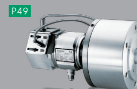
MS-C Non through-hole rotary hydraulic cylinder.(valve and switch brackets included)
