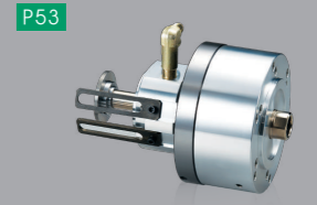
MRR Short type non through-hole rotary hydraulic cylinder. (for rotary union)
