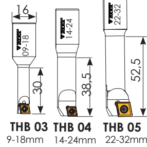
Cartridge
